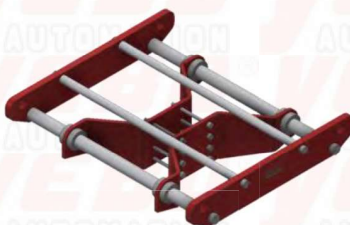
Trolley with 200mm stroke YBA-B007-200-L550-H200
