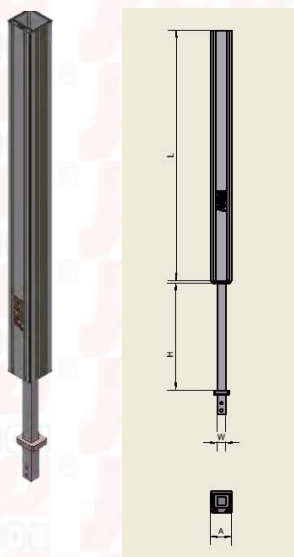
Standard Handy Lift
