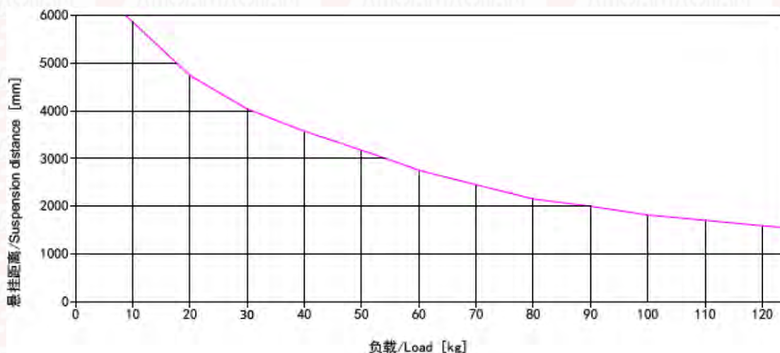
Load chart profile A065(For reference only)
