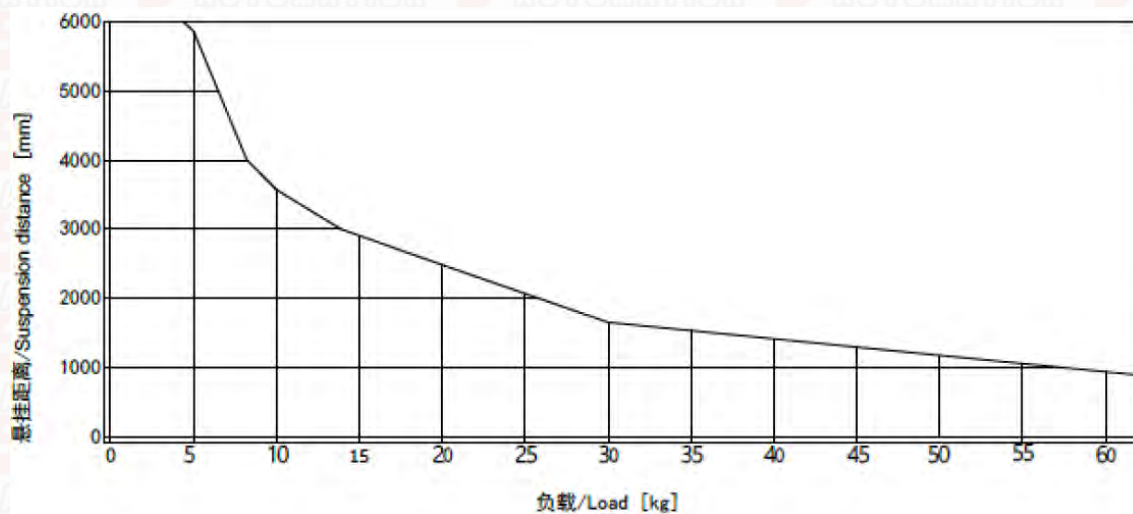
Load Chart Profile A055 (For reference only)
