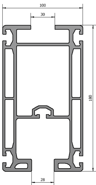
承载力数据图A180 (仅供参考) /Load chart profile A180(For reference only)
