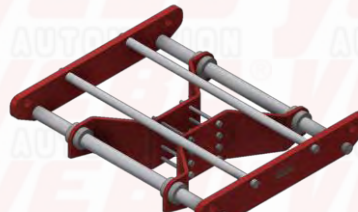
Trolley with 200mm stroke YBA-B007-200-L550-H200
